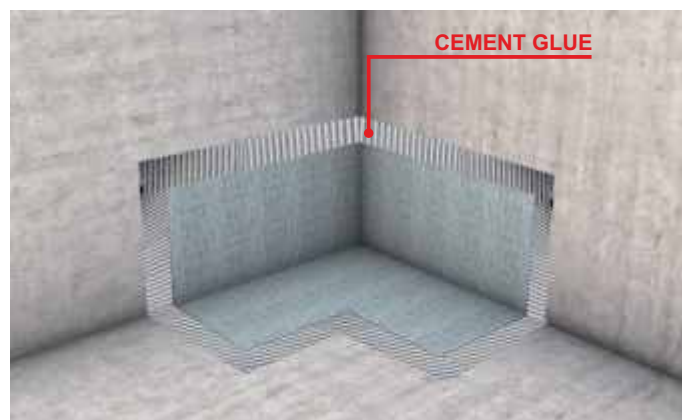
Example of installation of the waterproof sheet NOT ADHESIVE for internal corner use Art. 6813IM12C
